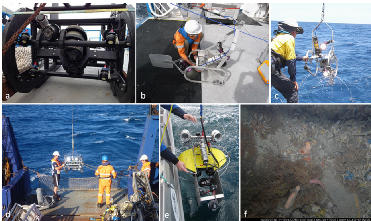
Figure 7.1: Types of towed camera systems deployed in Australian waters. a) MNFs Deep Towed Camera platform; b) and c) AIMS towed camera platform being deployed off RV Solander; d) towed camera platform being trialled by Geoscience Australia off RV Southern Surveyor; e) and f) Deakin University towed video system.
